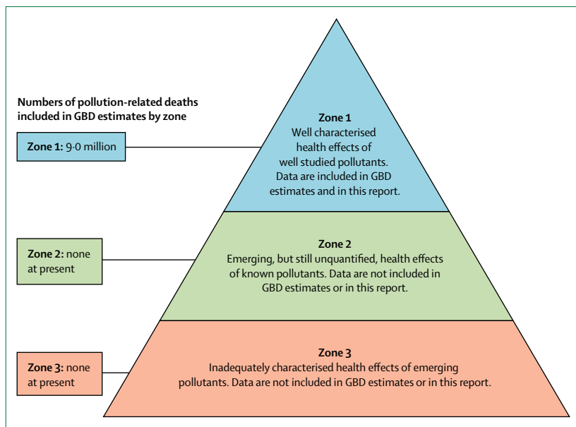
Figure 3: The pollutome
